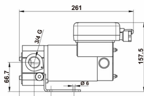
Viscomat 60/2
