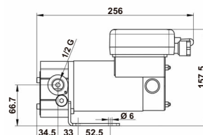
Viscomat 120/1
